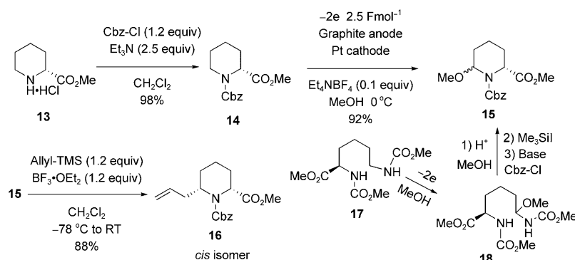
Scheme 3. Preparation of methyl (6 S )-allyl- N -benzyloxycarbonyl-D-pipecolate ( 16 ).
