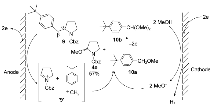
Scheme 2. Plausible electrochemical debenzylation route.
