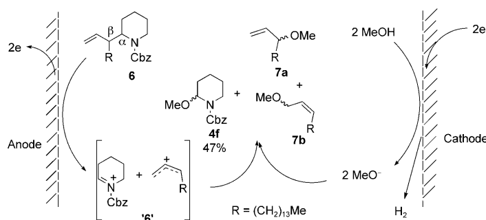
Scheme 1. Plausible electrochemical deallylation route.
